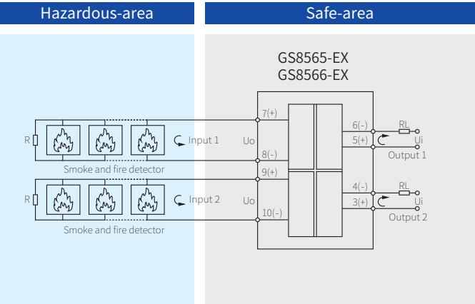
Note: GS8565-EX only contains input1, output1;
