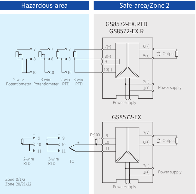
Note: a) 2-wire connection cannot eliminate conductor resistance and error will increase b) Bus-powered function is optional, if necessary please specified when ordering, and purchase bus power accessories in additional.
