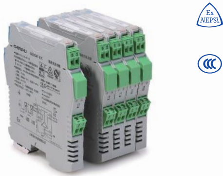
Dimensions: 118.9mm x 106.0mm x 12.5mm
